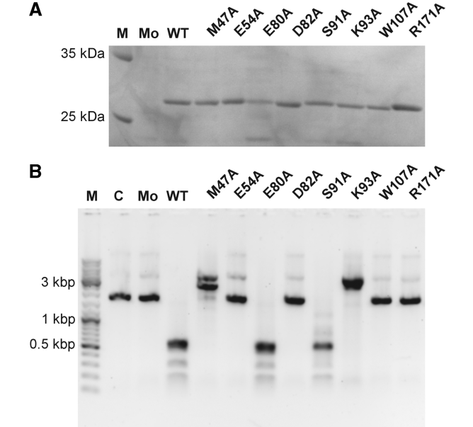
Figure 6. Enzymatic activity of the ThaI variants: (A) Coomassie stained SDS–PAGE gel proving that equal amounts (5 ng) of ThaI and its variants were used in the assay. (B) Electrophoresis of 600 ng pUC19 plasmid alone (control, ‘C’), incubated with E. coli lysate of cells not overexpressing ThaI (mock, ‘Mo’), or overexpressing ThaI or its variants (lanes 4–12). ‘M’ stands for the protein marker in panel A and for the DNA marker in panel B.
