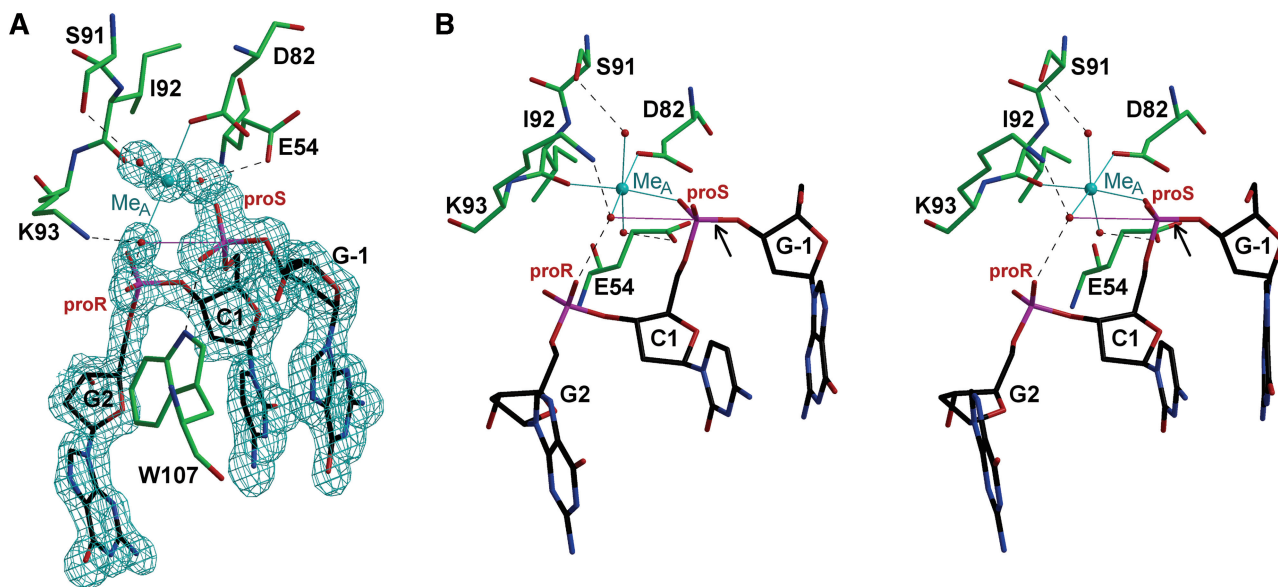
Figure 3. ThaI active site: (A) Mono representation of the ThaI active site showing the final composite omit electron density contoured at 1.5σ for the DNA, the metal ion and its coordinating water molecules. (B) Stereo representation of the active site highlighting the catalytic residues. In both panels, the interactions of the metal ion A (cyan) are shown as thin continuous lines and selected hydrogen bonds as dashed lines. The arrow in panel B marks the scissile bond. The orientation of panel B is consistent with Figure 1A.
