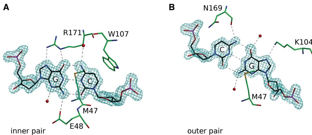
Figure 4. DNA sequence recognition by Tha I: hydrogen bonding interactions between Tha I and the specifically recognized bases of the inner (A) and outer (B) pairs are shown as dashed lines. The intercalating Met47 and wedging Trp107 are also included in the figure. The electron density is a final composite omit map contoured at 1.5\sigma .
